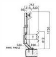
Barriera H4BP400P2250
