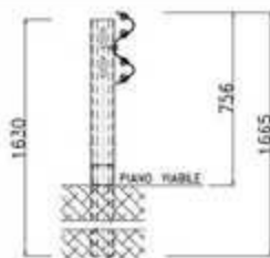
Barriera N2BL400
