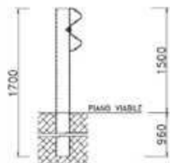
Barriera N2BL300
