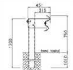
Barriera H2BL300
