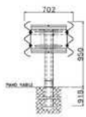
Barriera H4ST-R200
