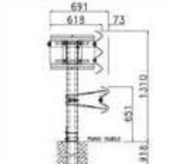
Barriera H4aBL100
