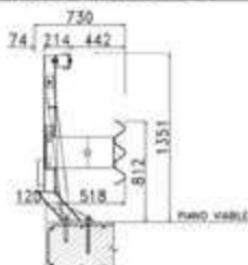
Barriera H2BP300-aus.
